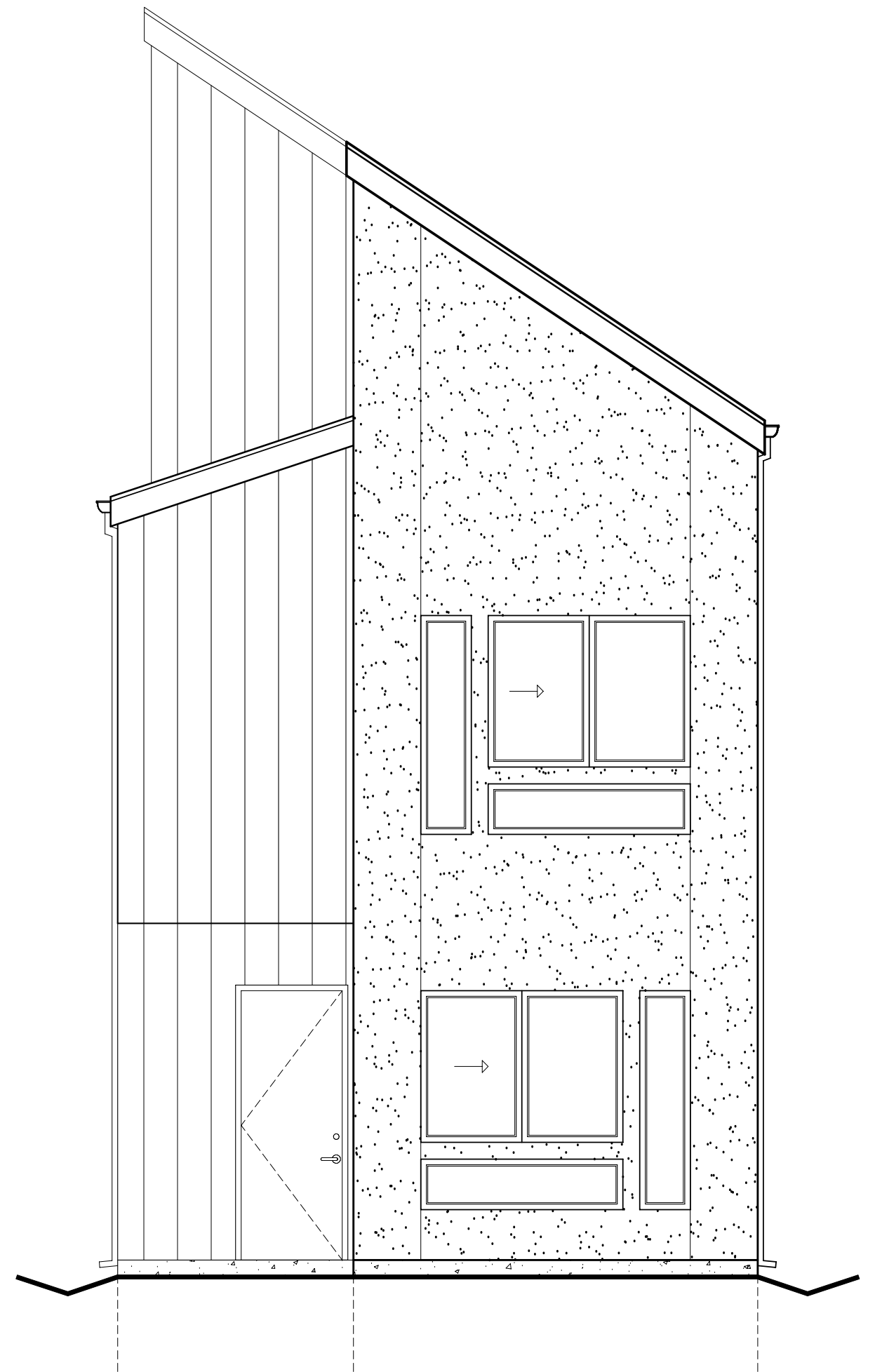
FRONT ELEVATION
