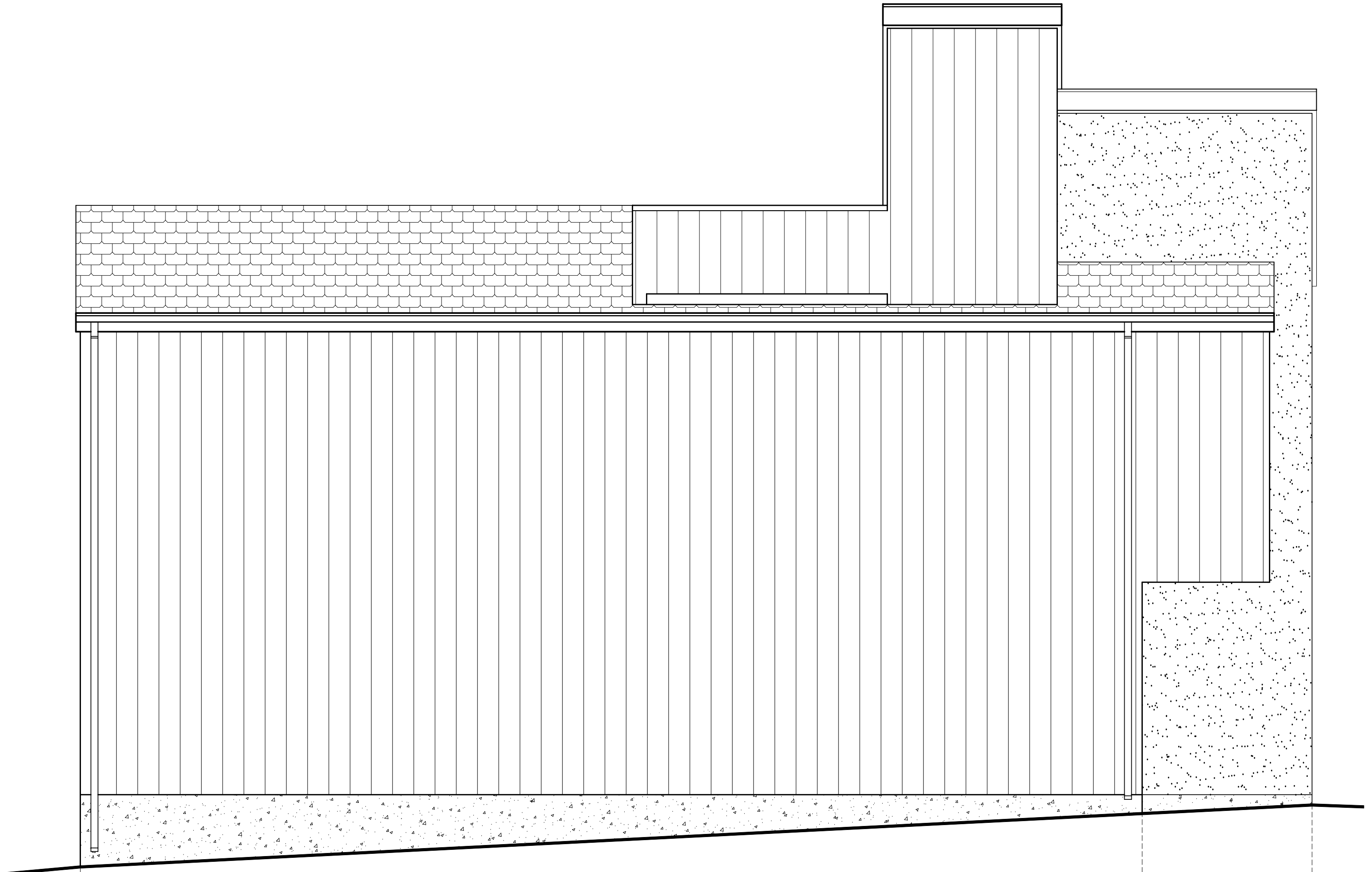
NORTH ELEVATION
